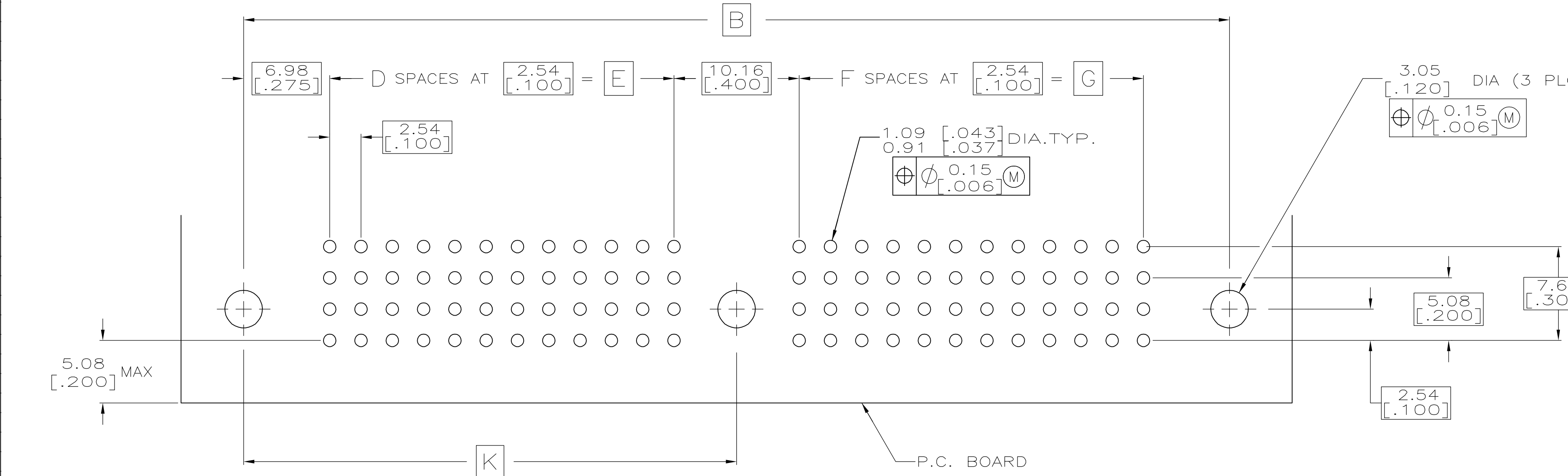
RECOMMENDED P.C. BOARD LAYOUT \triangle
